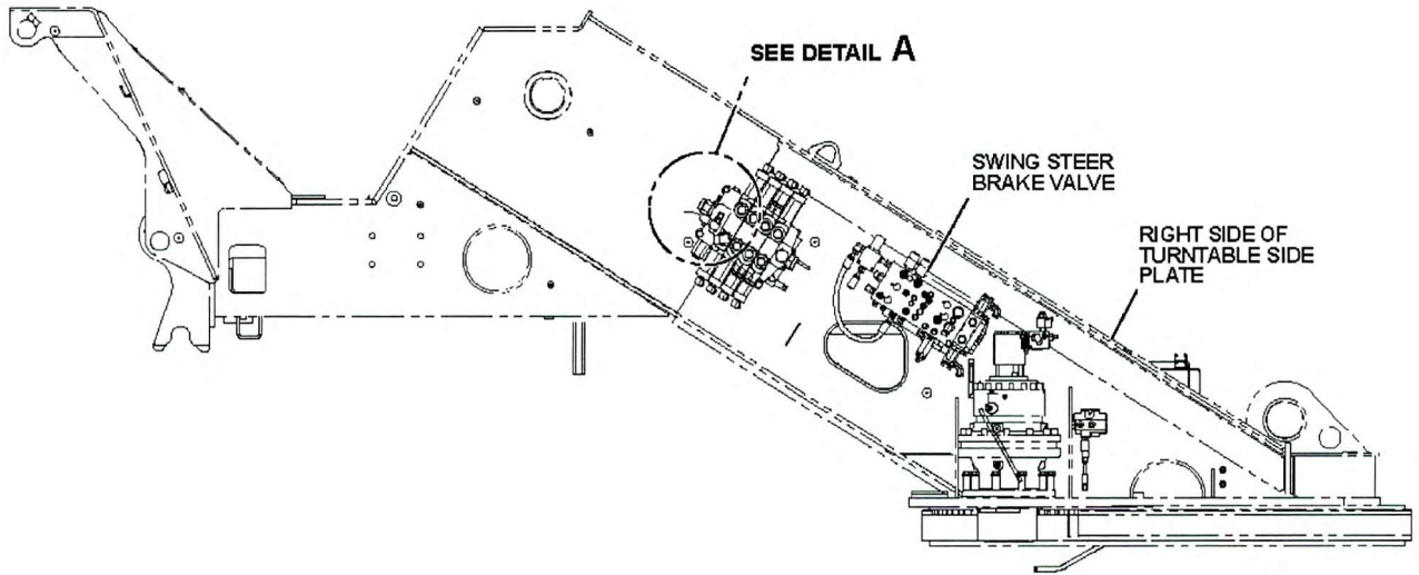
VALVE INSTALLATION VIEW
