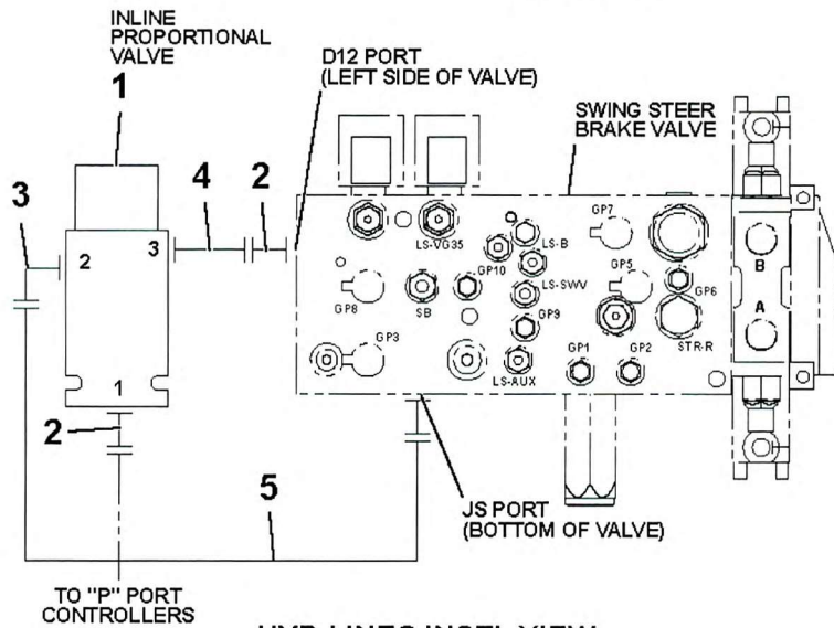
HYD LINES INSTL VIEW
